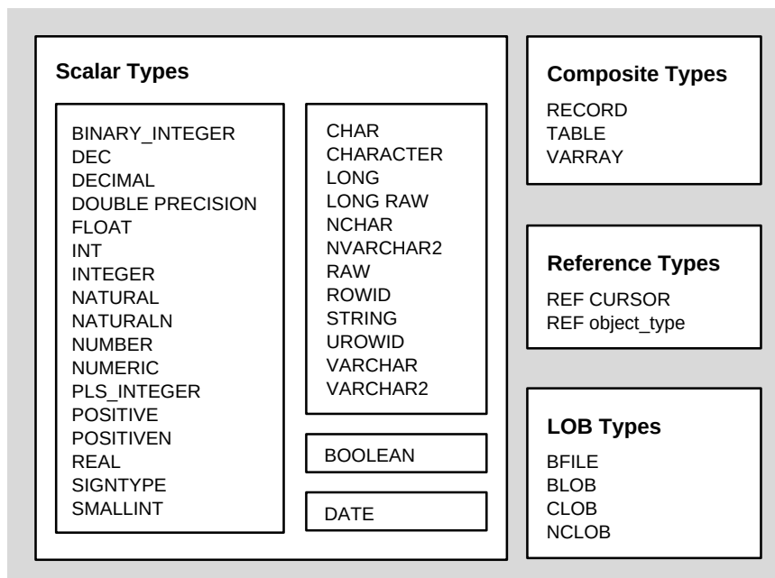
Figure 2–1 Built-in Datatypes
