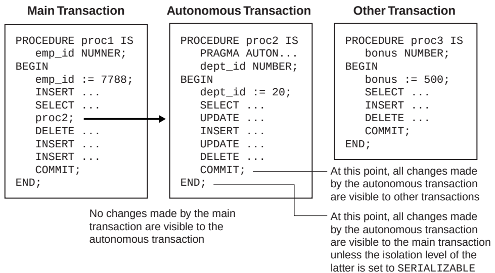
Figure 5–3 Transaction Visibility
