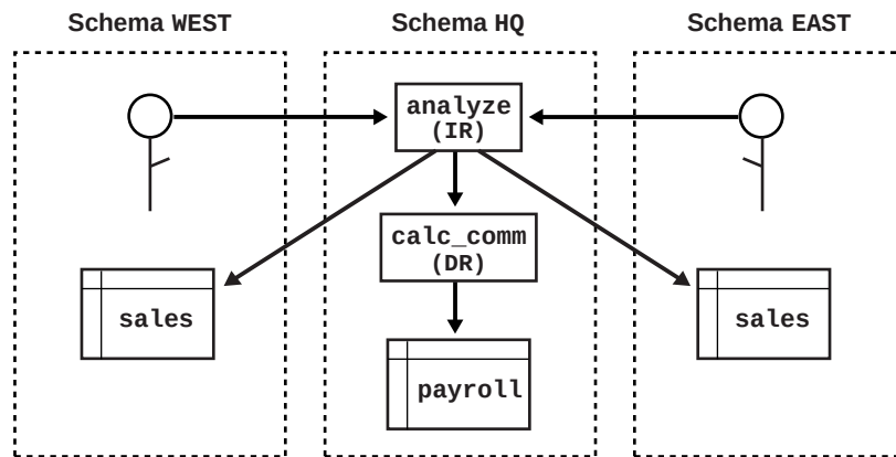
Figure 7-4 Controlled Access
