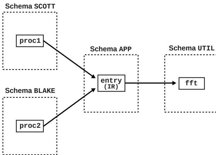
Figure 7-5 Indirect Calls
