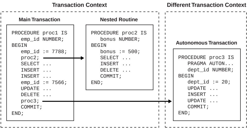
Figure 5–2 Transaction Context
