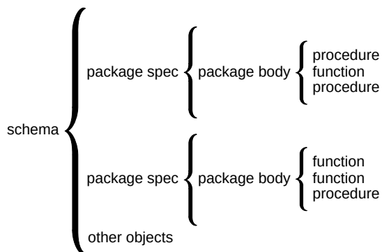
Figure 8–2 Package Scope
