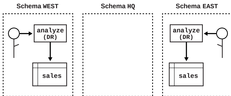
Figure 7-2 Definer-Rights Problem
