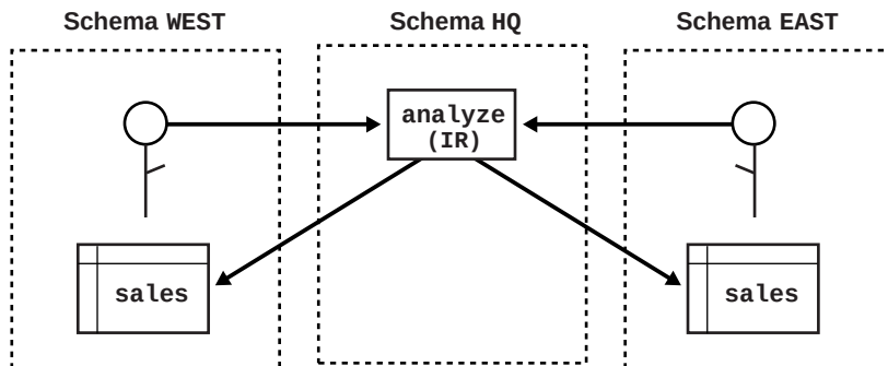
Figure 7-3 Invoker-Rights Solution
