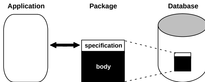
Figure 8–1 Package Interface
